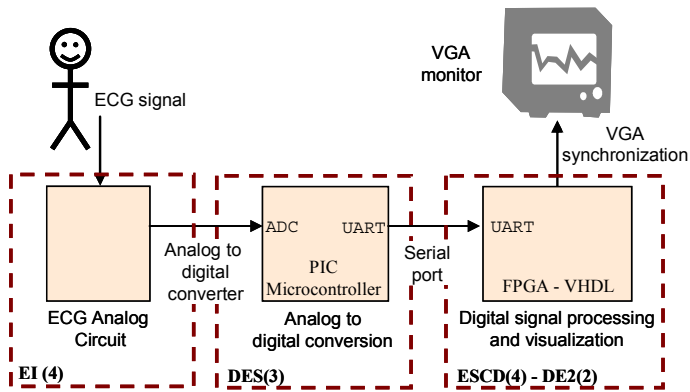
Figure 7: Basic ECG project
