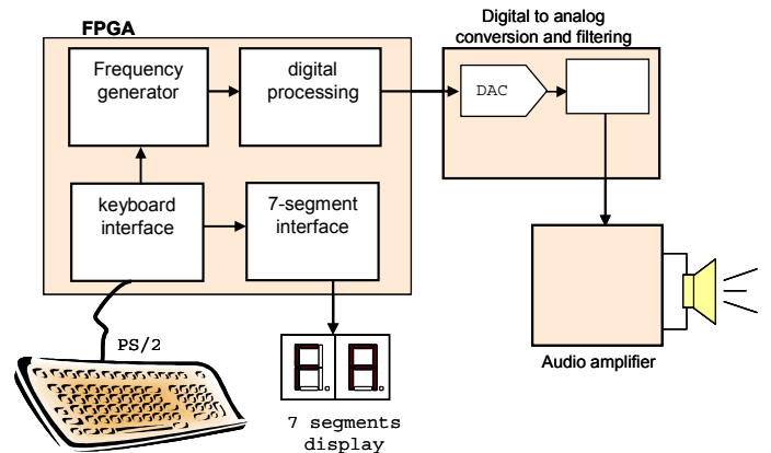
Figure 6: Proposals for the enhanced electronic piano project
