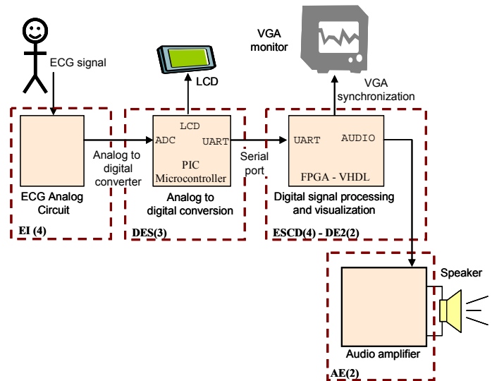
Figure 8: Enhanced ECG project
