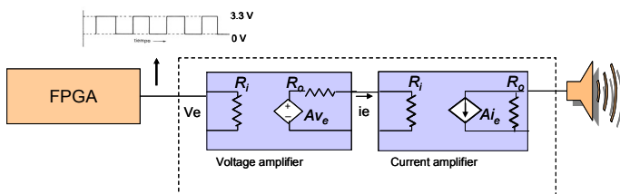
Figure 5: General scheme of an amplifier
