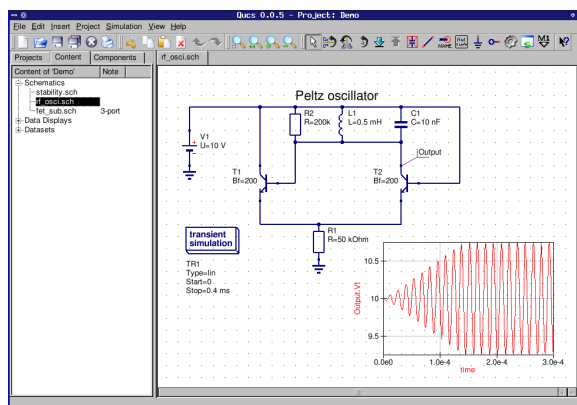
Figure 2. Screenshot of Qucs, taken from [16]
